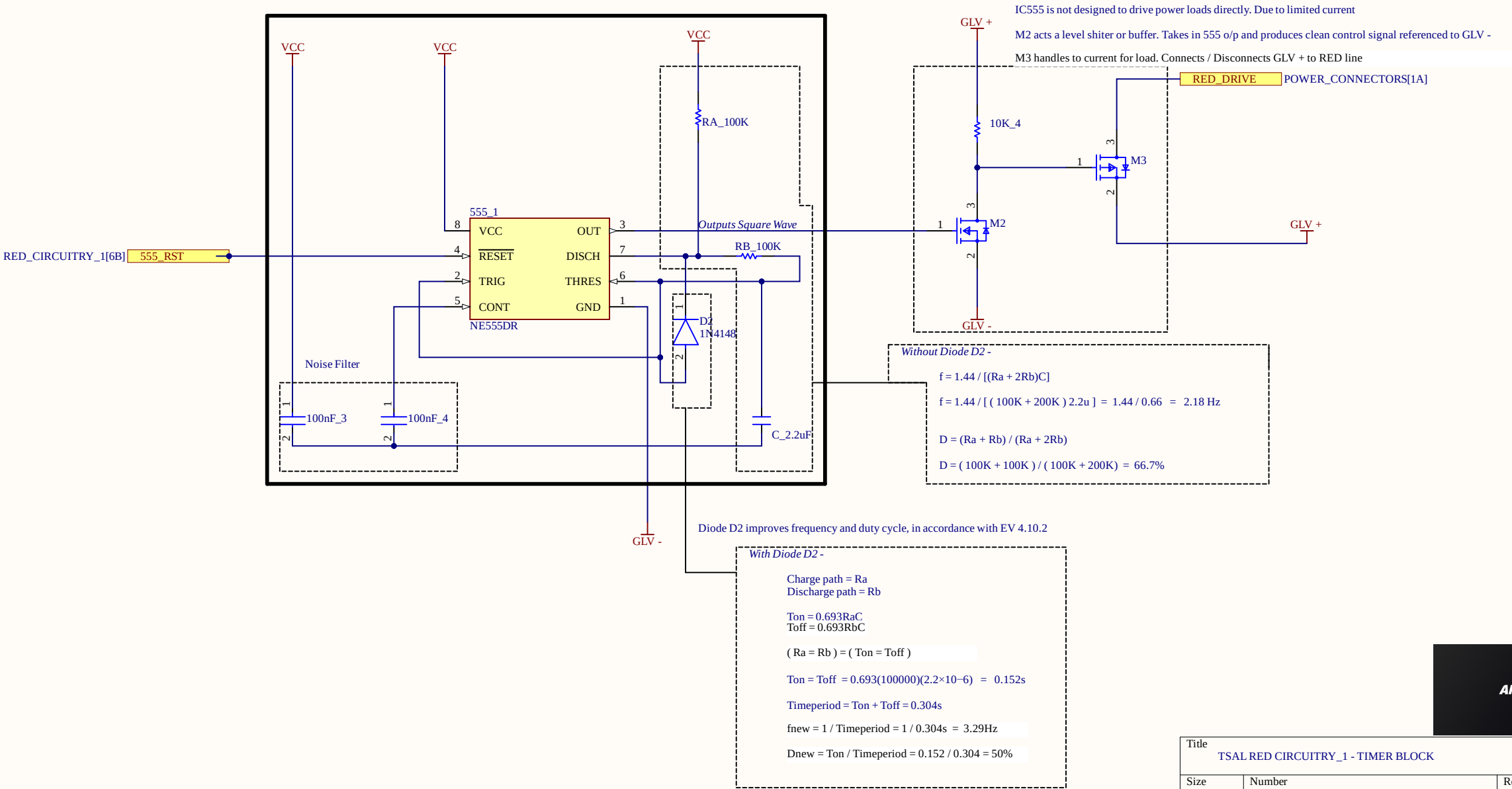
IC 555 Timer in Astable Multivibrator Configuration
